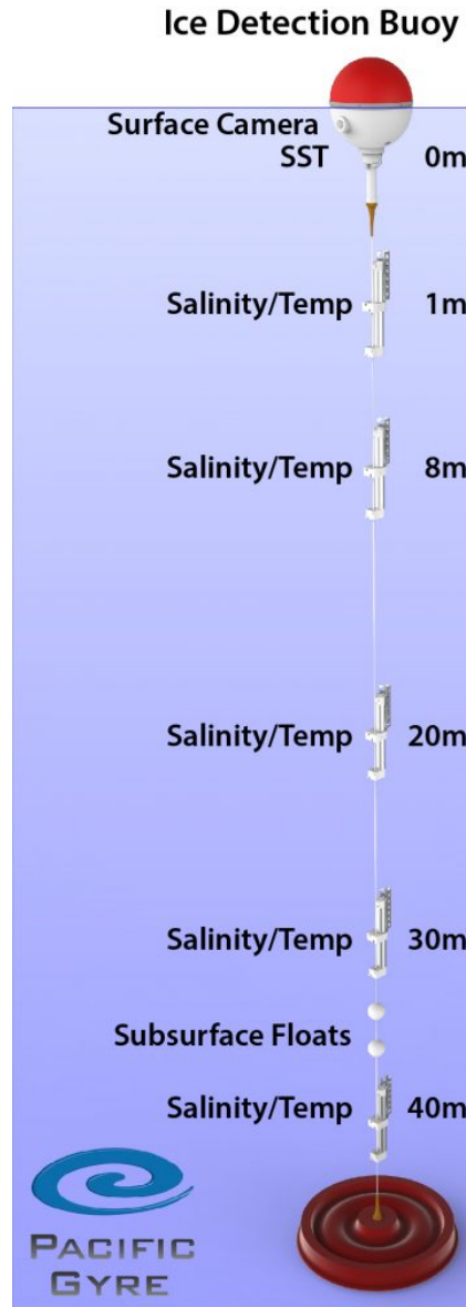
Difference between sea water temperature and freezing point at 4801730 - Chukchi Ice Detection Buoy (degree_Celsius_difference)
