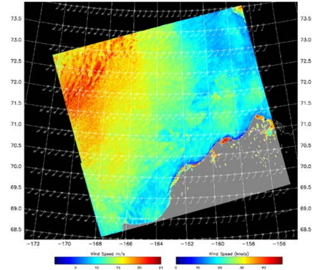
SAR Wind: RSAT2_GSS_2017_11_08_04_08_25_0563429305_162.96W_71.37N_J4I_CS_GFS05CDF_wind_Level2.nc
